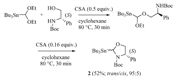
Scheme 4. Optimised synthesis of oxazolidines 2-trans .
