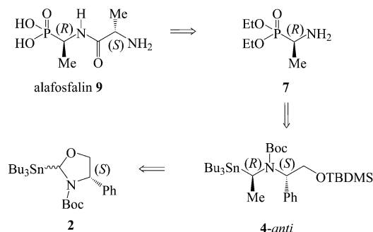
Scheme 2. Retrosynthesis of alafosfalin.
