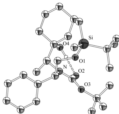
Figure 1. Molecular structure of compound ent-5a-anti (hydrogen atoms are omitted for clarity).
