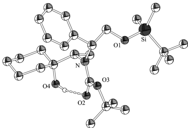
Figure 2. Molecular structure of ent-5a-syn (hydrogen atoms are omitted for clarity).
