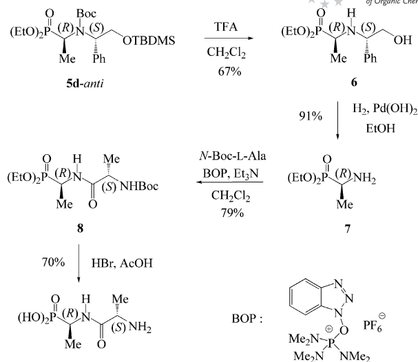
Scheme 7. Synthesis of alafosfalin.
