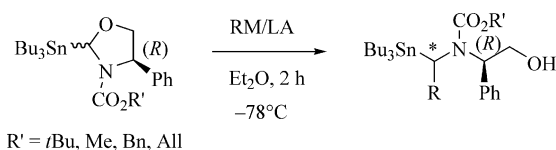
Scheme 1. Diastereoselective ring opening of 2-tributylstannyl-1,3-oxazolidines by organometallic reagents.
