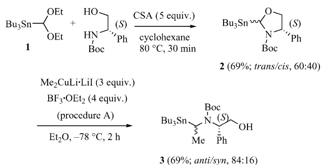
Scheme 3. Synthesis of tributylstannylated \alpha -amino alcohols 3 via oxazolidines 2 .
